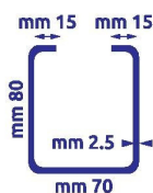
barra perimetrale perimetrical beam
